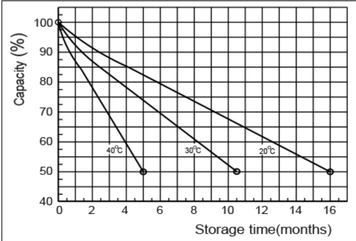
SELF-DISCHARGE CHARACTERISTICS
