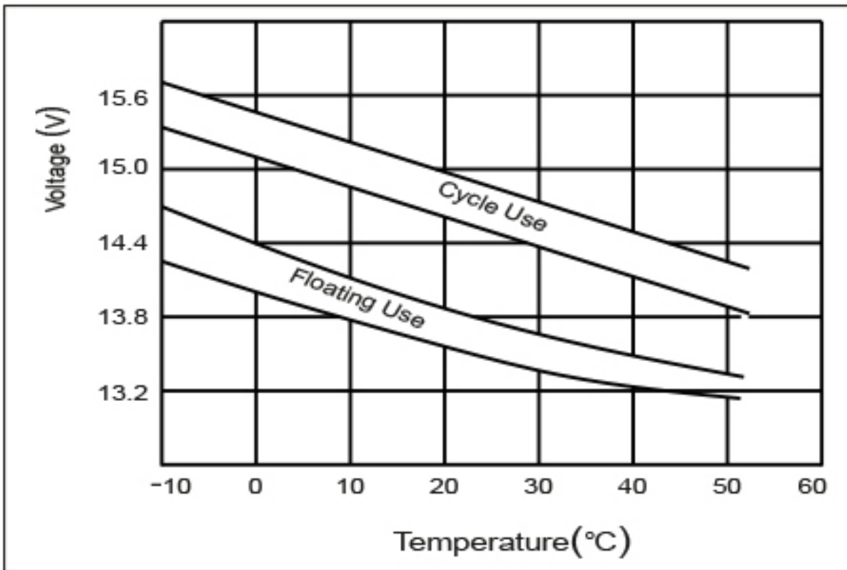
THE RELATIONSHIP FOR CHARGING VOLTAGE AND TEMPERATURE
