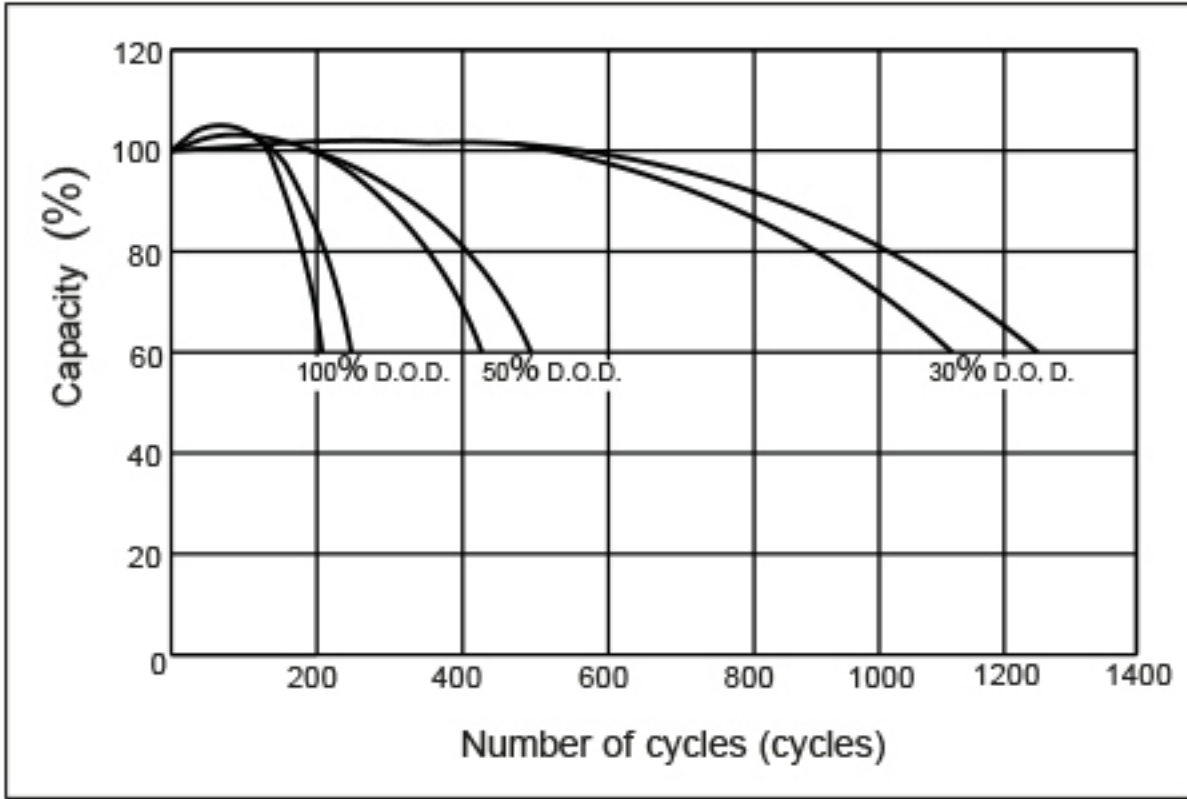
CYCLE LIFE ON D.O.D (25°C)
